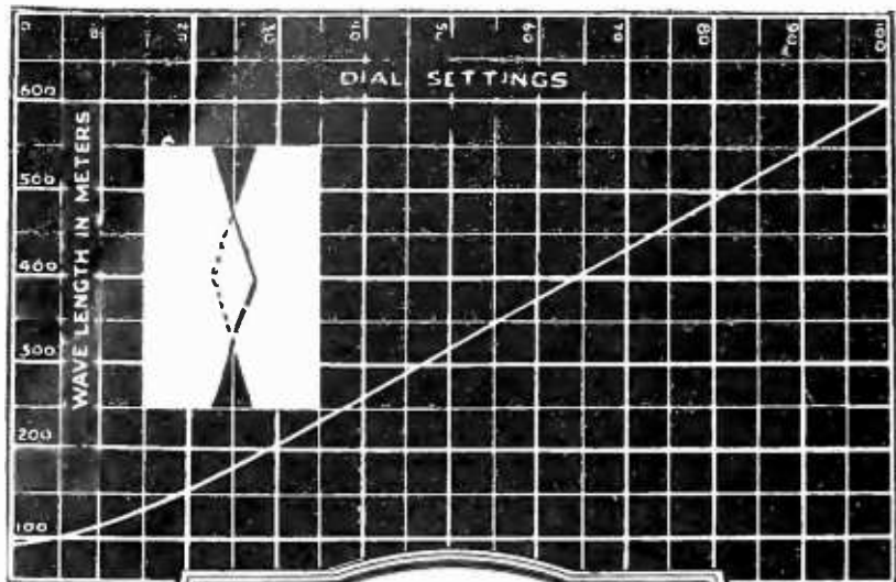
Curve of WADE .005 mfd. Square Law Condenser showing Straight Line Wave-Length and Wide Tuning Range.
