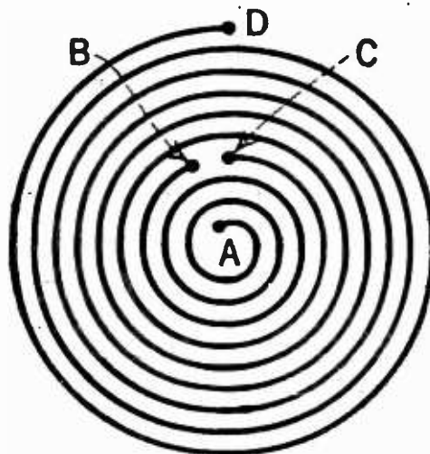
A B = PRIMARY C D = SECONDARY
